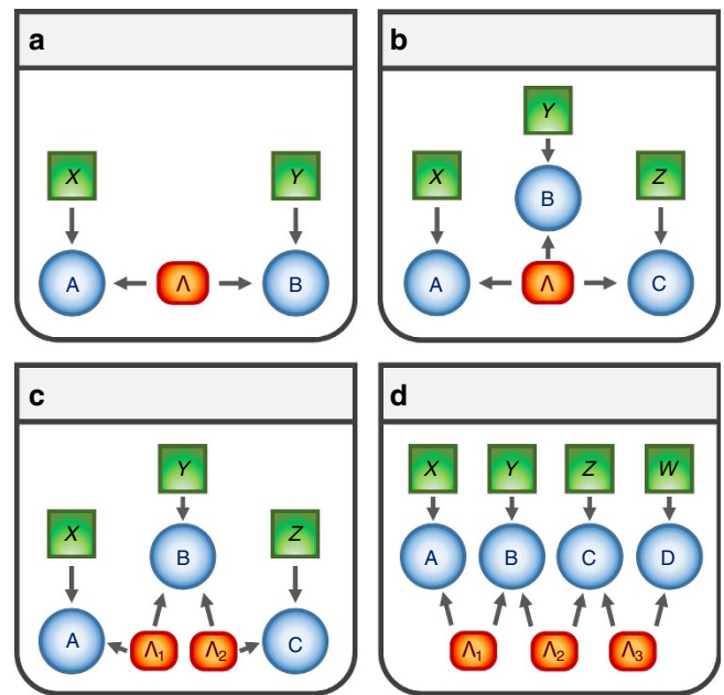
Figure 1 | Representation of the causal structures underlying the networks 45 . Directed acyclic graphs 45 can represent different causal structures, for instance the nodes in the graph represent the relevant random variables with arrows accounting for their causal relations. There are three different kinds of nodes: hidden variables (orange boxes), measurement settings (green boxes) and measurement outcomes (blue boxes). (a) Bipartite LHV model. (b) Tripartite LHV model. (c) Tripartite scenario with two independent LHVs, that is, bilocal hidden variable (BLHV) model. (d) Possible extension of the bilocal model to a linear chain of four stations with three independent LHVs.
