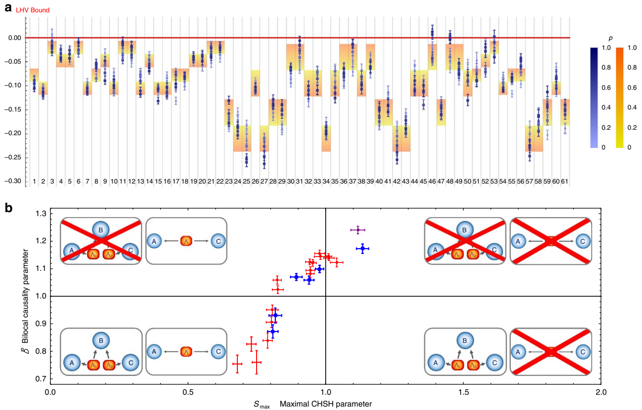
Figure 4 | Experimental test of LHV models. (a) Experimental violation values for all the 61 Bell inequalities compatible with a LHV model. Each column corresponds to a different inequality, where a resulting value > 0 is not compatible with an LHV model. Each point’s colour represents the estimated amount of noise p , from dark blue ( p=1 , that is, absence of noise), to light blue ( p=0 , that is, maximum noise). Theoretical predictions are shown in the background, the red to yellow colour transition representing the dependence from p . Squares (circles) represent those points, which violate (do not violate) the bilocal causality inequality (equation (3)). (b) Comparison between experimental bilocal causality parameter and maximized CHSH parameter (multiplied by a factor 1/2 so that the local bound of the CHSH inequality is set to 1) in different regimes of noise. Bilocal causality test is performed with fixed non-optimized measurement settings, whereas CHSH maximum parameter is computed applying the Horodecki criterion (ref. 30) to a partial quantum state tomography (red points) or a complete quantum-state tomography (blue points) of the quantum state shared between A and C after the entanglement swapping protocol (that is, conditioned on singlet state outcome in station B). The purple point was evaluated directly testing both bilocal causality and CHSH in a particular regime of low noise. Circles (squares) represent entangled (separable) quantum states, where the degree of entanglement was computed via the partial transpose 46 . The lower-left region is compatible with both models, the upper-left region denotes incompatibility with bilocal causality, the upper-right region denotes violation of both the bilocal causality and CHSH inequalities, whereas the lower-right region is characterized by only CHSH violation. Error bars indicates 1 s.d. of uncertainty, due to Poissonian statistics.
