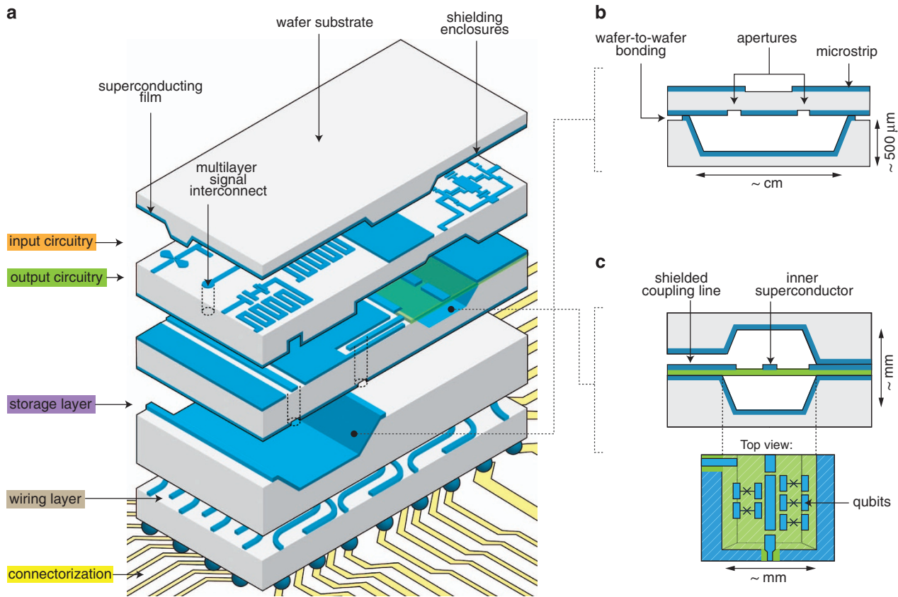
Figure 2. Proposed schematic of a multilayer microwave integrated quantum circuit (MMIQ). (a) Layers are made of silicon wafers with features etched out of the bulk using micromachining techniques to create enclosures that serve as high-Q resonators and as shielding for internal components. Superconducting metallisation (blue) covers the walls of these enclosures and enables low-loss wafer-to-wafer bonding of the layers. Dense planar input/output circuitry, including filters, switches and amplifiers can be embedded in other layers. RF and DC vertical interconnects carry signals between layers, and wire-bonding or ball-grid connection can be used to interface with external control and measurement electronics. (b) A cross-section of the rectangular cavity resonator shows interlayer aperture coupling between the cavity and transmission lines above. (c) 3D superconducting transmission lines could be constructed using membranes (green) in the micromachined structure. Some of these can be populated with qubits and act as a compact low-loss quantum bus.
