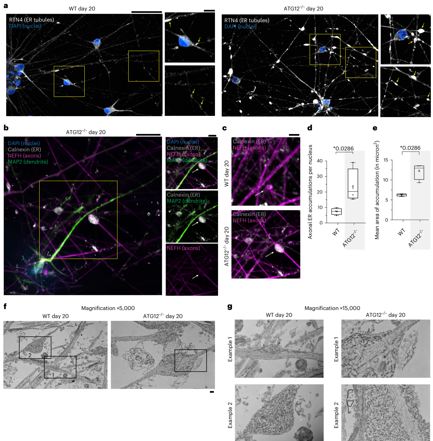
Fig. 2 | Autophagy-dependent clearance of ER in axons during iNeuron differentiation. a , WT or ATG12 -/- day-20 iNeurons immunostained with ER-tubule marker \alpha -RTN4 (white) and with DAPI (nuclei, blue). Scale bars, 50 \mu m (full images) and 10 \mu m (zooms). b , Enlarged ER-positive structures in ATG12 -/- day-20 iNeuron axons revealed by immunostaining with \alpha -calnexin, ER (white); \alpha -MAP2, dendrites (green); \alpha -NEFH, axons (magenta); and DAPI, nuclei (blue). Scale bars, 10 \mu m (full image) and 5 \mu m (zooms). c , As in b , day-20 iNeurons were immunostained with \alpha -NEFH and \alpha -calnexin to identify aberrant ER structures; here we compare the zoomed-in region of axons in ATG12 -/- iNeurons to a similar region for WT iNeurons. Scale bar, 5 \mu m. d , Min-to-max box-and-whiskers plot for the number of axonal ER accumulations per nucleus, where the box represents the 25th to 75th percentiles, whiskers extend from min to max values, the line
