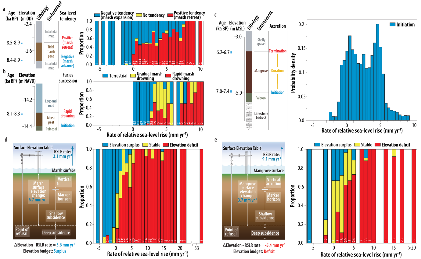
Extended Data Fig. 2 | Details of individual studies from which the probabilities of marsh and mangrove vertical adjustment to RSLR were inferred. (a) Analysis of tidal marsh retreat and advance recorded in sediment archives from across the United Kingdom 15 . (b) Analysis of marsh drowning recorded in sediment archives from the Mississippi Delta 16 . (c) Analysis of global mangrove accretion recorded in sediment archives from 12 . (d) Analysis of surface elevation tables (SET) from global tidal marshes 29 . (e) Analysis of surface elevation tables (SET) for mangrove SET sites in Extended Data Table 2.
