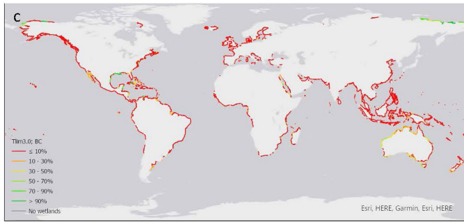
Extended Data Fig. 6 | Inland retreat potential of existing mangrove and tidal marsh. Percentage of the current wetland area that could potentially be compensated for via wetland inland retreat until 2100, calculated for two sea-level rise scenarios. Median projections for 2.0 °C warming, allowing
