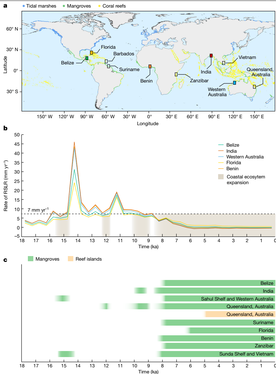
Fig. 1 | Coastal ecosystem responses to RSLR following the Last Glacial Maximum. a , Present-day distribution of mapped coastal ecosystems and the location of case studies highlighted in b, c . b , Median rates of RSLR over time derived from GIA modelling (Methods). c , Timing of habitat advance and
