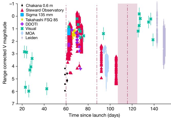
Fig. 1 | The reflective brightness of BW3 as a function of days since launch. The data points represent the range-corrected magnitudes, where the brightness was scaled using an inverse square law of the range versus orbital height, to provide numerical values ‘as seen’ at local zenith. The shape and colours represent the different observations: Ckoirama Observatory’s Chakana telescope (black circles), Steward Observatory SSA astrograph (red triangles), complementary metal-oxide-semiconductor (CMOS) camera Sigma 135 mm lens (light blue squares), Oukaïmeden Observatory Takahashi FSQ 85 (yellow stars), Deca-Degree Optical Transient Imager (DDOTI; purple plus signs), visual (green crosses), MOA-II (grey-blue diamonds) and Leiden (grey circles). The vertical brown dot-dash lines from left to right are the times corresponding to the unfolding of the array (60 days since launch), the beginning of dimming (85 days since launch) 8 and our estimate of the start of brightening ( 117.75 \pm 8.75 days since launch) based on the observations, where the shaded region denotes the uncertainty because of observing cadence. In some cases, the error bars are smaller than the data point size and represent the Poisson distribution of the integrated flux of the satellite trail in the image. All uncertainties are 1 s.d.
