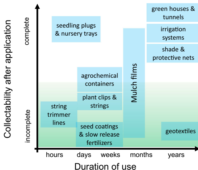
Fig. 3 Collectability and duration of use of plastics in agriculture.
