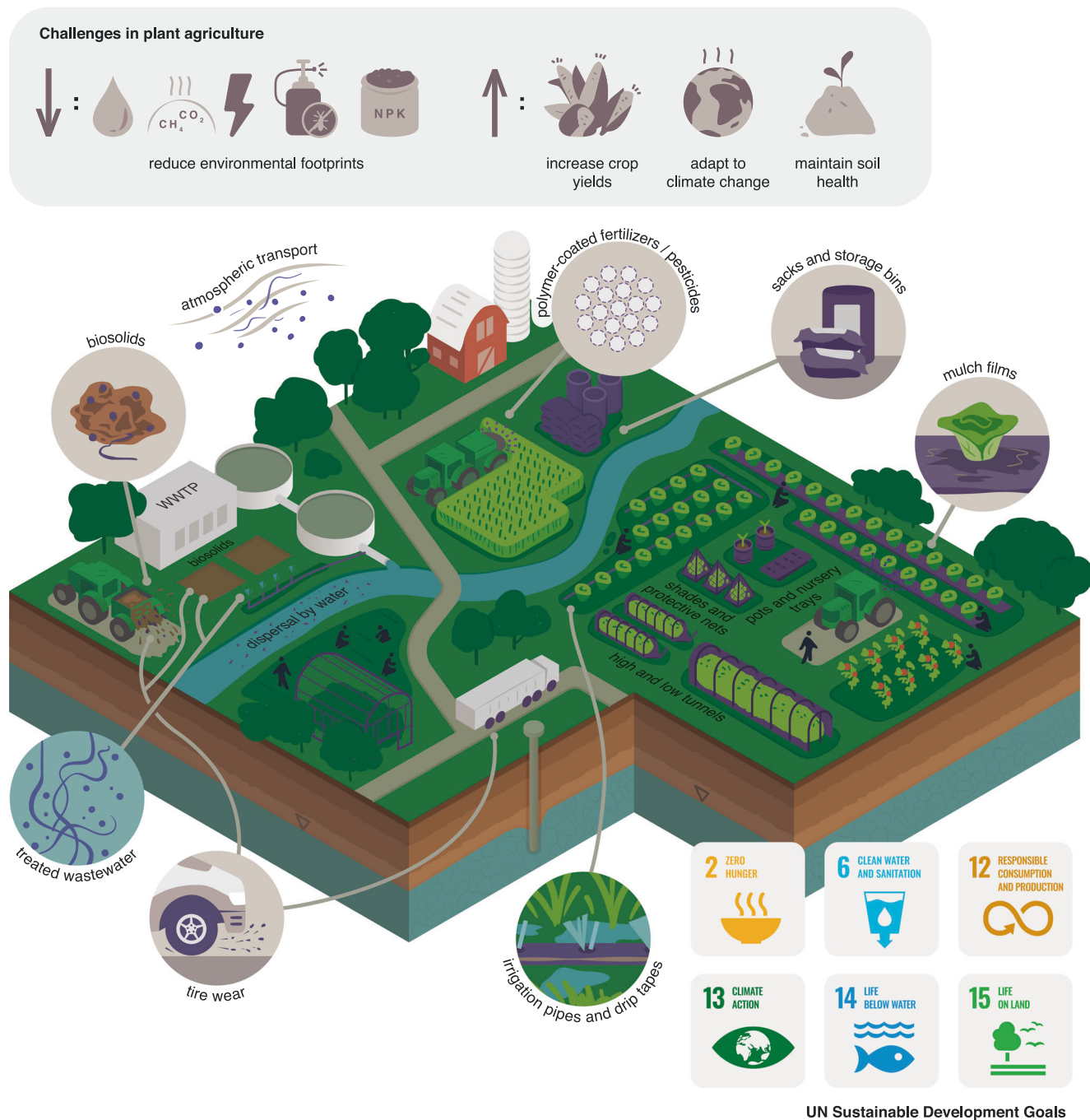
Fig. 1 Applications of plastics in plant agriculture. There are multiple applications of plastics in plant agriculture. Plastics help to reduce irrigation water, pesticide, and fertilizer demand, leading to reduced greenhouse gas emissions and increased crop yield, which impacts several UN Sustainable Development Goals. There are also diverse sources of incidental plastic pollution on croplands; for example, during the dispersal of wastewater biosolids or treated wastewater from wastewater treatment plants (WWTP), including tire wear particles contained therein.
