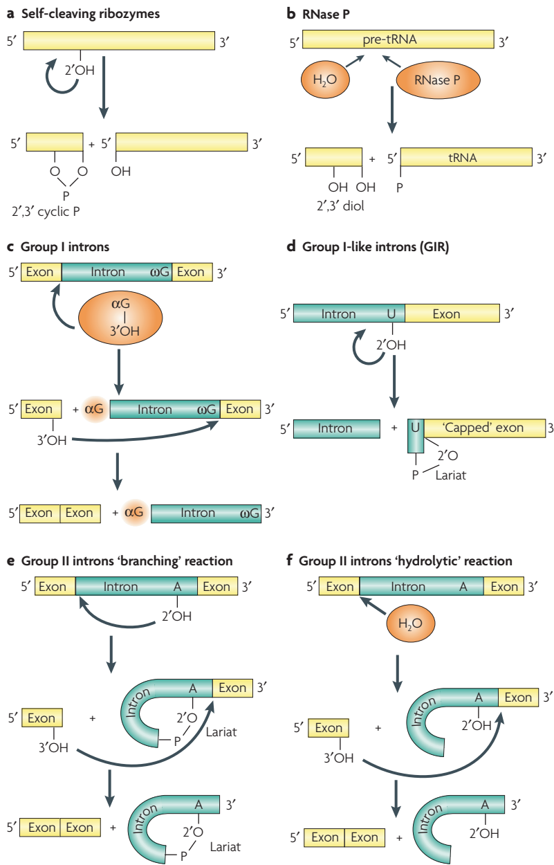
Figure 2 | Reactions catalysed by ribozymes. a | The typical reaction of self-cleaving ribozymes, initiated by 2'-hydroxyl (OH) attack, and yielding 2',3'-cyclic phosphate (P) and 5'-OH termini. b | The catalytic cleavage of pre-tRNA by RNase P (REF. 2). A water molecule serves as a nucleophile, and the reaction yields 2',3'-diol and 5'-P termini. c | Self-splicing by group I introns 1 . The reaction is initiated by nucleophilic attack by the 3'-OH of external guanosine ( \alpha G) at the 5' splice site. This results in covalent linkage of \alpha G to the 5' end of the intron and release of the 3'-OH of the 5' exon. In the second step, the 3'-OH attacks the 3' splice site located immediately after the conserved guanosine ( \omega G), resulting in excision of the intron with \alpha G at the 5' end and release of the ligated exons. d | The 'capping' reaction of the Didium iridis GIR1 ribozyme is similar to the first step of the 'branching' reaction of group II introns 25 . The reaction joins nucleotides by a 2',5'-phosphodiester linkage, thereby forming a 3-nucleotide 'ariat' that might be a protective 5' cap of the mRNA. e | The self-splicing of group II introns by a branching reaction 22 . In the first step, the 5' splice site is attacked by the 2'-OH of a conserved unpaired adenosine located in domain VI, resulting in formation of a 2',5'-phosphodiester linkage. In the next step, the free 3'-OH group of the 5' exon attacks the 3' splice site, liberating the circular intron lariat and ligated exons. f | Alternative 'hydrolytic' self-splicing of group II introns 22 . The reaction involves a water molecule as a nucleophile and produces a linear intron.
