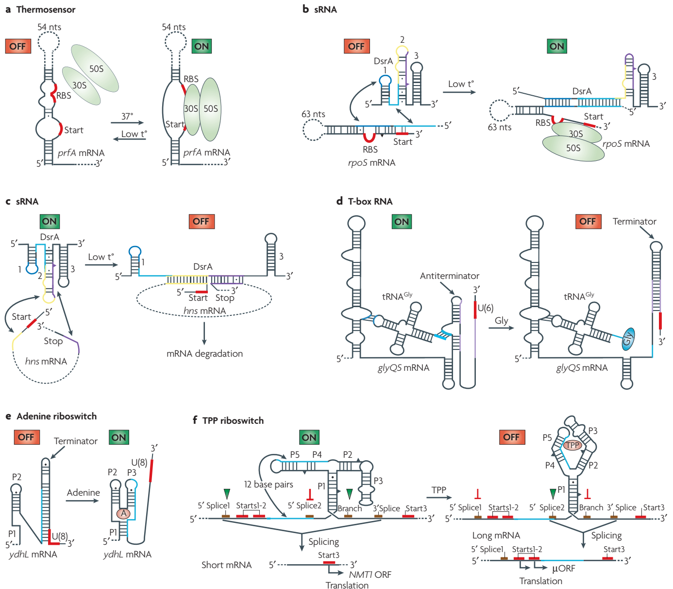
Figure 3 | Gene regulation by RNA switches. RNA regions that are involved in gene expression switching are shown in the same colour. a | Translation activation of virulence genes in the pathogen Listeria monocytogenes 28 . An increase in temperature melts the secondary structure around the ribosome binding site (RBS) and start codon, allowing ribosome binding and translation initiation. b | Upregulation of Escherichia coli \sigma^5 -factor gene by the DsrA antisense short RNA (sRNA). DsrA RNA 121 pairs with the translational operator of the rpoS gene 122 using two sequences (coloured blue and light blue) located within helices 1 and 2 (REFS 33,34, 121). This base pairing exposes translation initiation signals for ribosome binding and increases mRNA stability 101 . c | Downregulation of transcription regulator HNS by DsrA sRNA. DsrA RNA, transcribed in response to low temperature, pairs with 5' and 3' regions of hns mRNA and causes faster turnover of the mRNA 101 , possibly by RNase E degradation 123 . d | Transcription termination of the Bacillus subtilis glycyl-tRNA synthetase gene by aminoacylated tRNA Gly (REF. 124). Non-aminoacylated tRNA Gly interacts with the T-box region of mRNA using an anticodon and an acceptor helix 125 , and promotes the formation of the anti-terminator stem-loop structure. The aminoacylated tRNA cannot contact mRNA using the acceptor stem, thus allowing the formation of the transcription terminator. e | Transcription activation of
